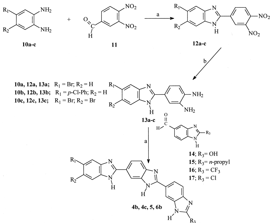
Scheme 1. (a) \text{PhNO}_2 , 145^\circ\text{C} ; (b) \text{Pd/C} ; \text{H}_2 or \text{NiAl} (Ra-Ni); \text{EtOH} .
